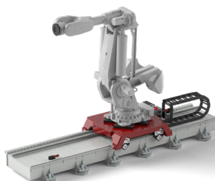
TMF-5 floor-mounted linear track with ABB industrial robot
