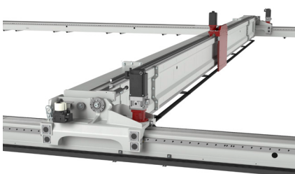
Y-axis (bridge)
